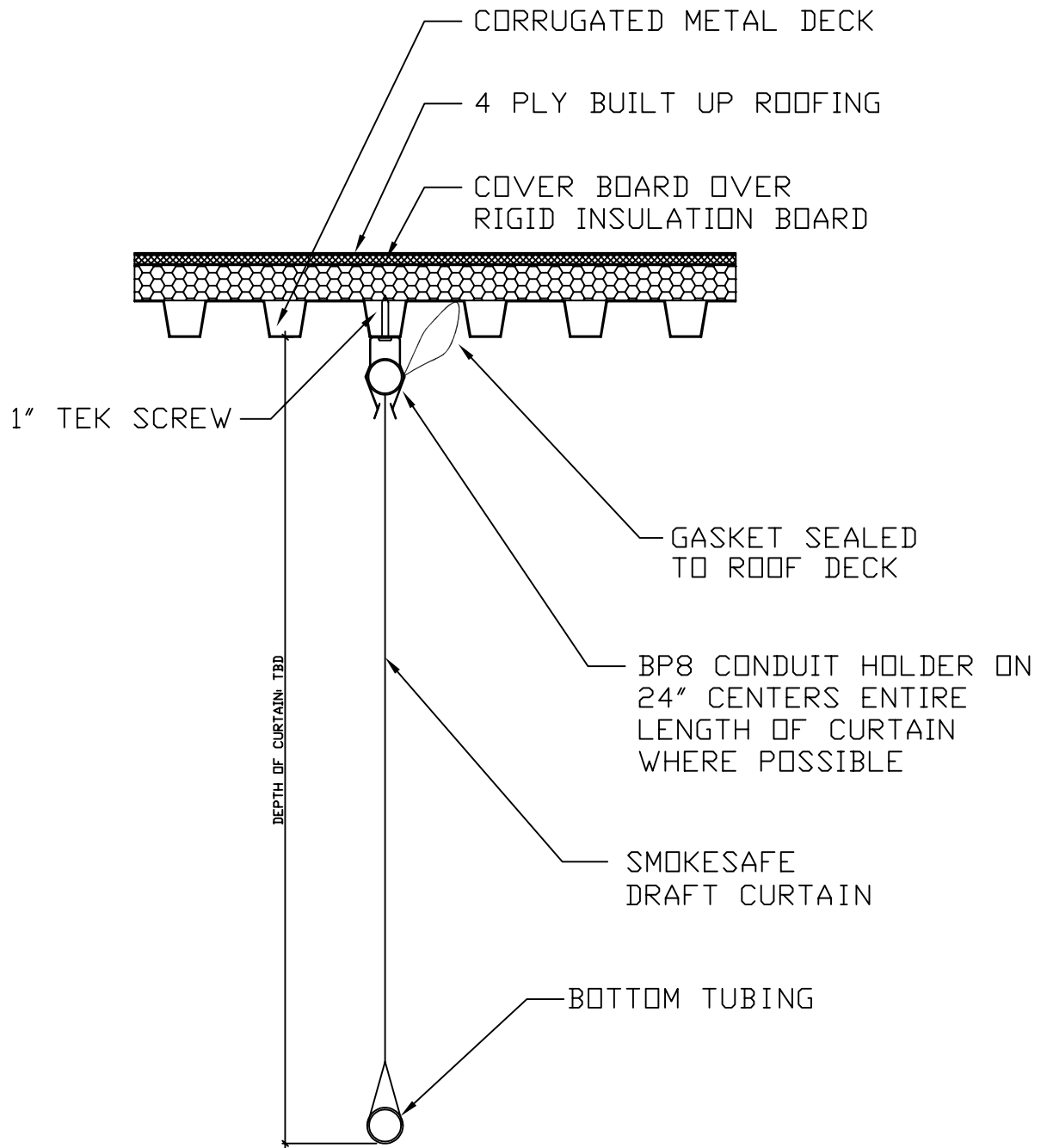
DRAFT CURTAIN SECTION CONNECTION ELEVATION ROOF DECK CONNECTION
